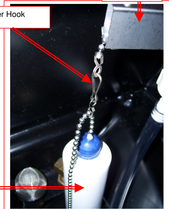
Float Valve
